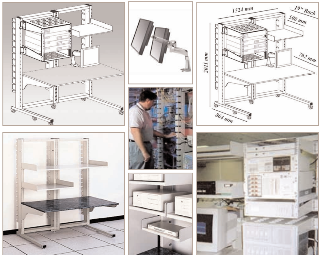
Console Rack Lan 60" (1524 mm)
